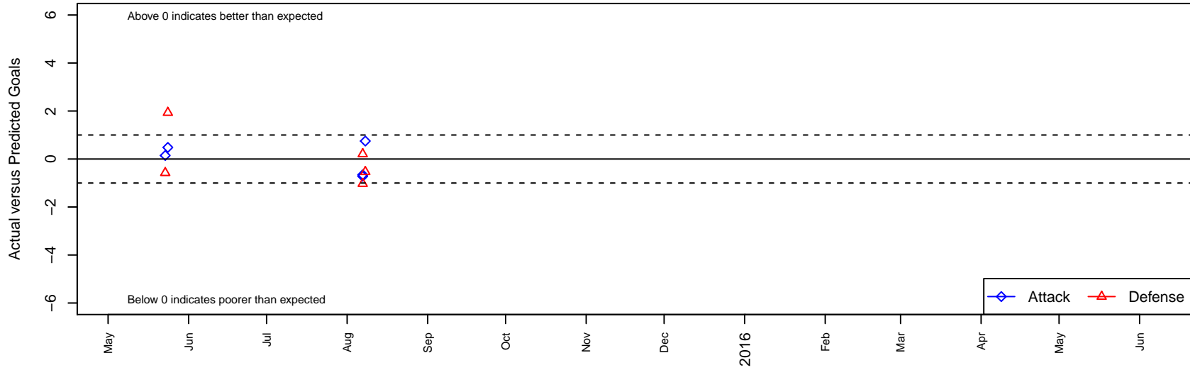
De Anza Force SC Blue B99 Dots are actual minus expected GF (blue circles) and GA (red triangles). Blue line is smoothed change in attack strength. Red is smoothed change in defense strength.
